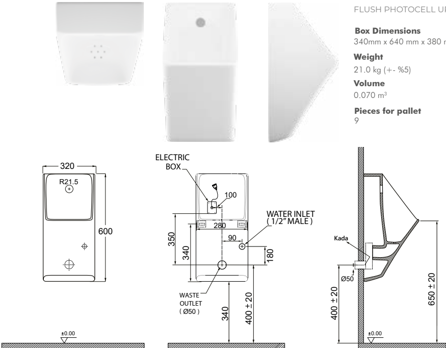
FLUSH PHOTOCEL URINAL & SEPARATOR FOTOSELLİ PİSUVAR & ARABÖLME
