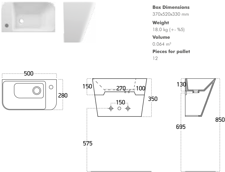
WALL HUNG MONOBLOCK WASHBASIN
