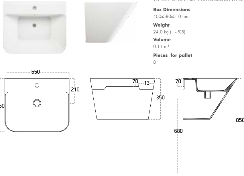
WALL HUNG HALF MONOBLOCK WASHBASIN
